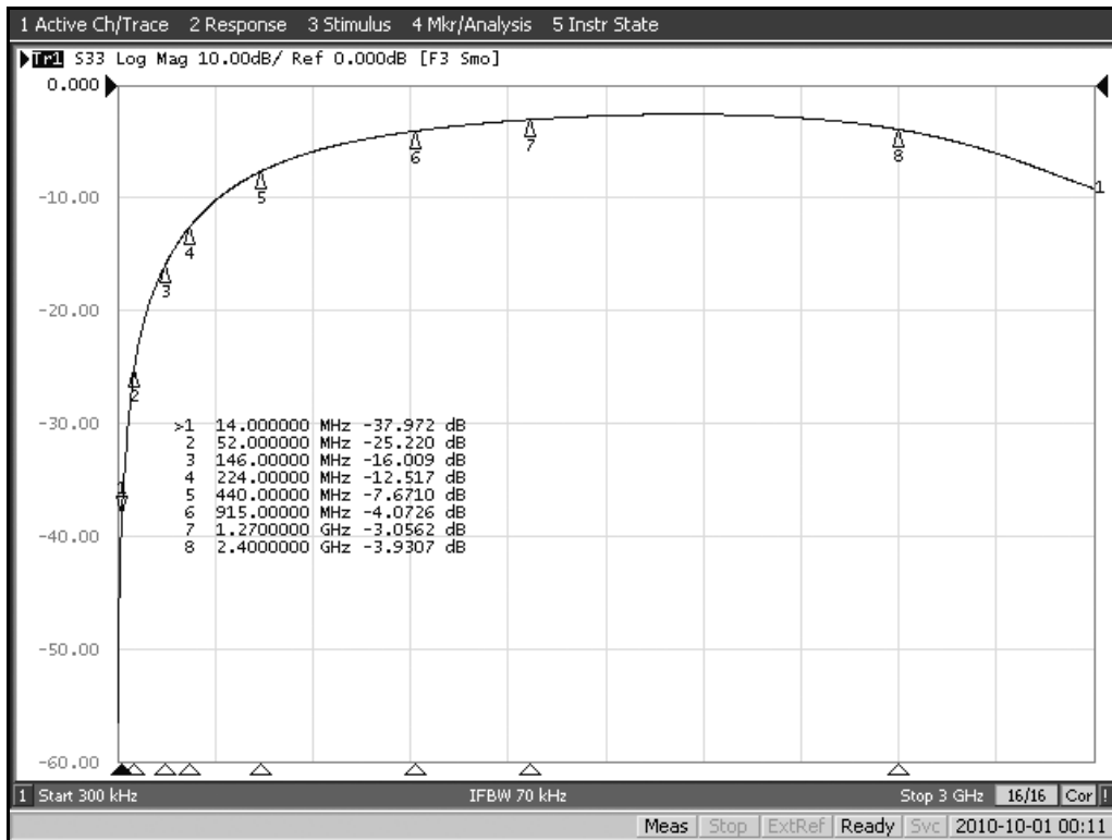
Figure 3 - Return loss
