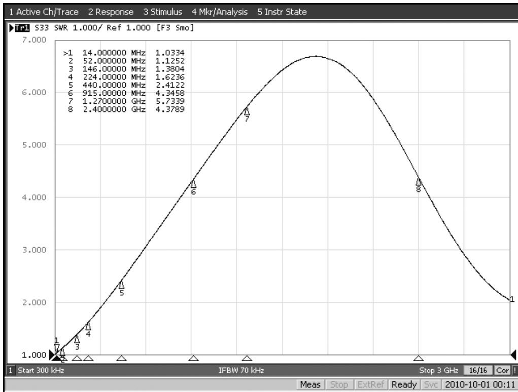
Figure 4 – VSWR
