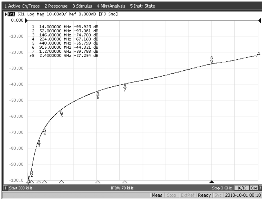
Figure 2 - Element rotated for minimum coupling
