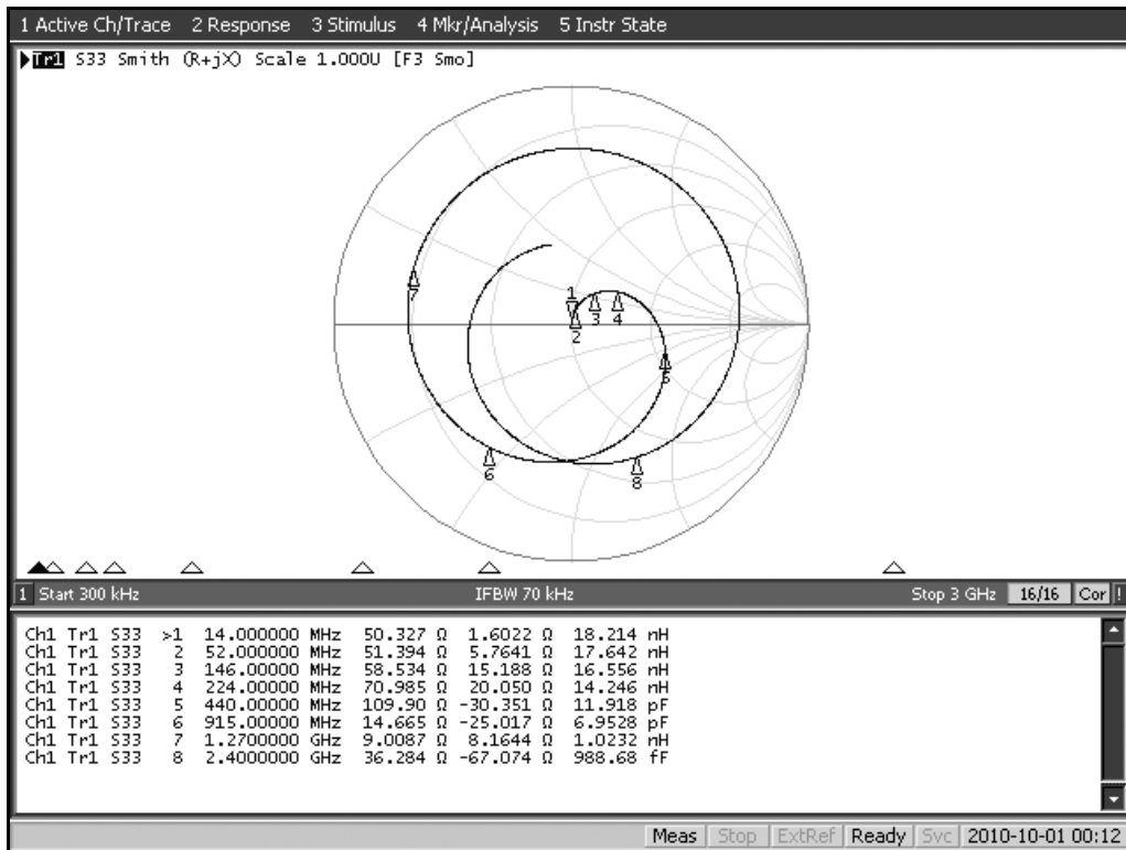
Figure 5 – Smith Chart
